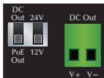
Figure 2-3: VC-203PT rear panel Figure 2-3: VC-203PR rear panel
