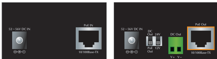
Figure 2-3: VC-203PT rear panel Figure 2-3: VC-203PR rear panel
