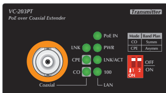
Figure 2-1: VC-203PT front panel
