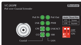
Figure 2-2: VC-203PR front panel
