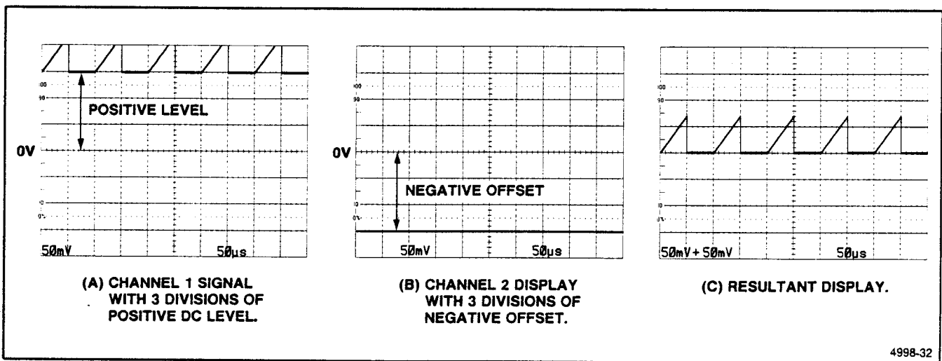
Figure 6-3. Algebraic addition.
