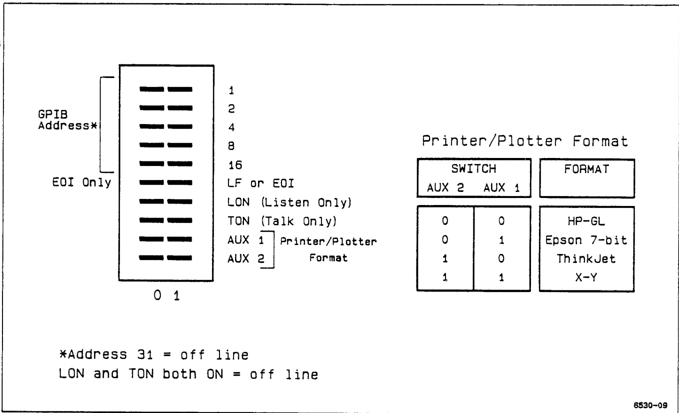
Figure B-16. Option 10 GPIB Interface PARAMETERS switch.
