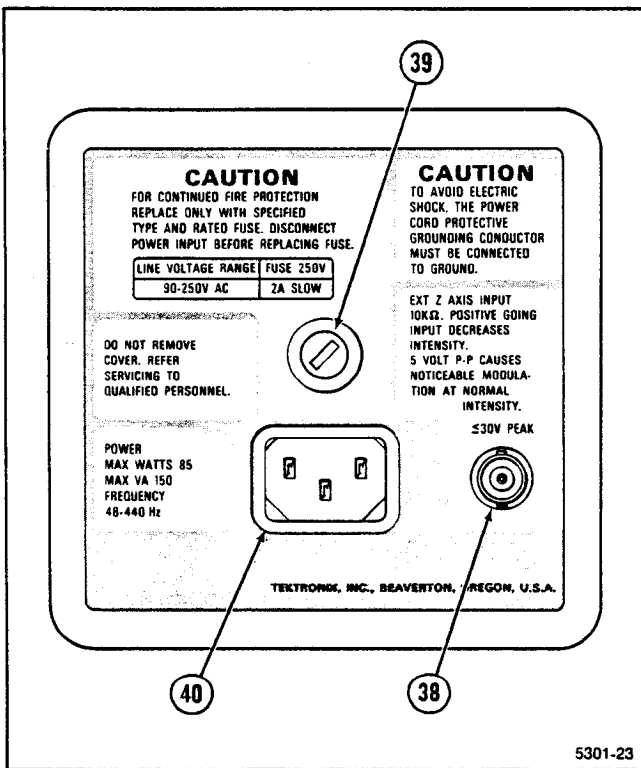
Figure 3-6. Rear Panel.
