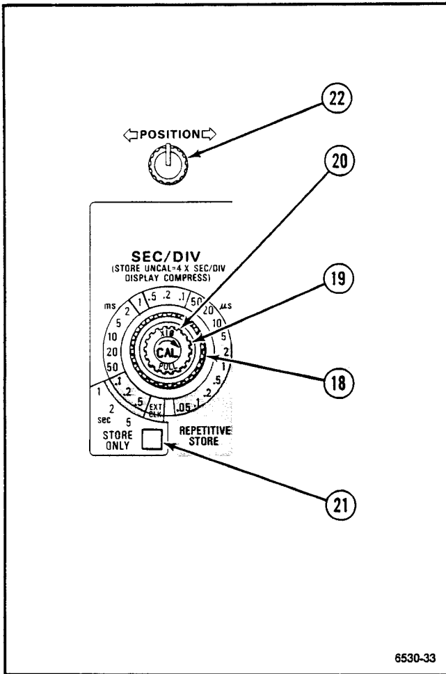
Figure 3-3. Horizontal controls.
