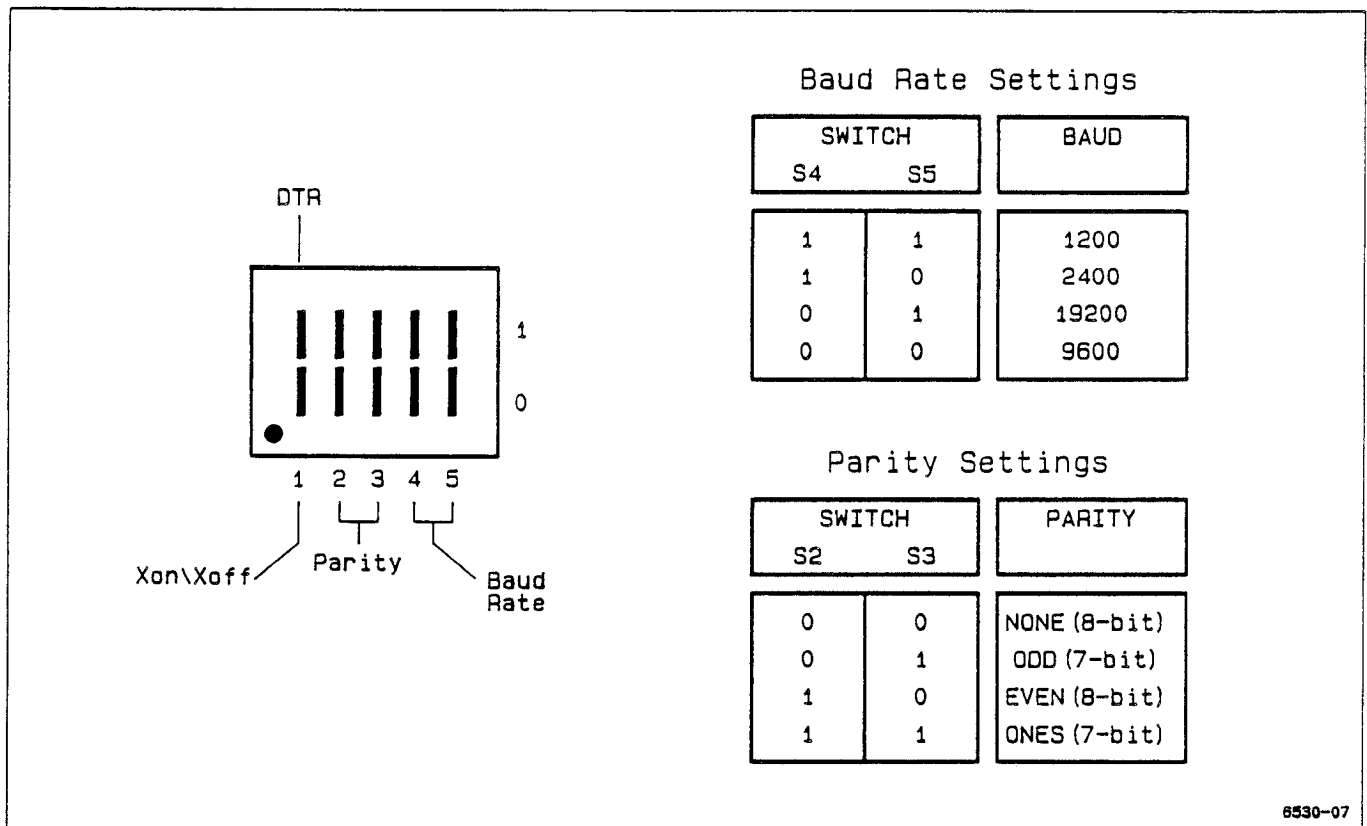
Figure B-14. HP ThinkJet RS-232-C switch settings.
