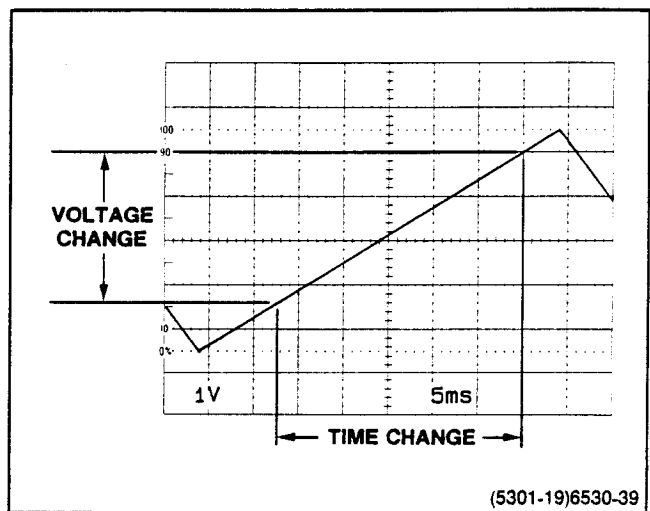
Figure 6-11. Slope.
