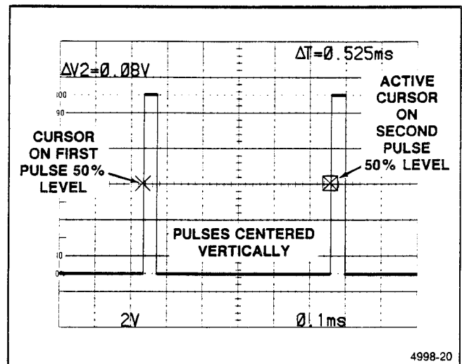
Figure 6-18. Time difference between repetitive pulses.
