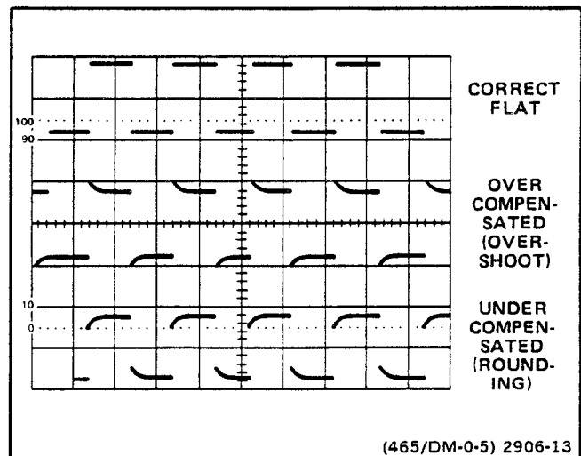
Figure 5-1. Probe compensation.
