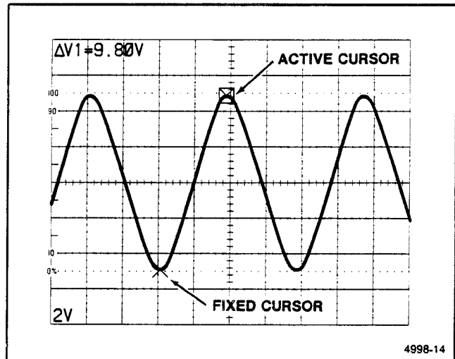
Figure 6-12. Ac peak-to-peak voltage, cursor method.
