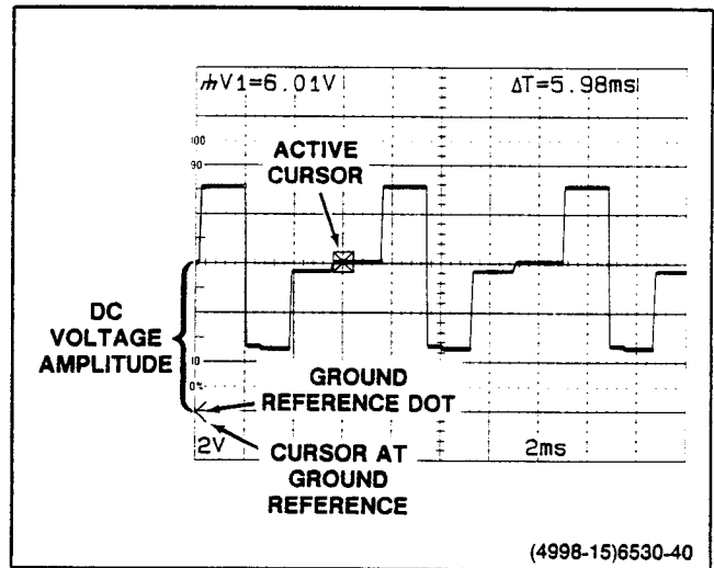
Figure 6-13. Ground referenced dc voltage, cursor method.
