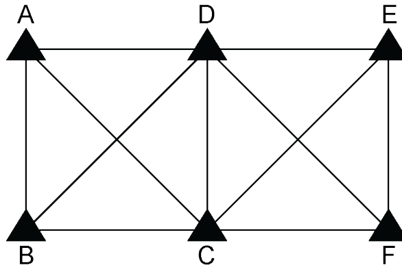
Figure 4: Trivial Baselines
