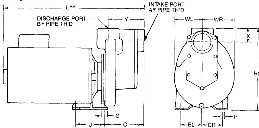
Figure 1 — Dimensions
