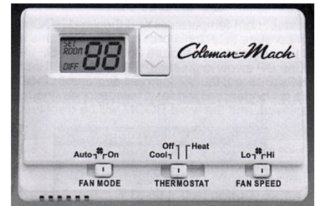
Figure 3-3. Thermostat
