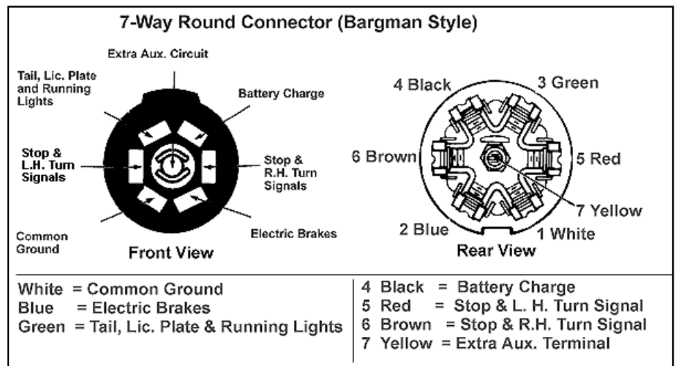
Figure 7-16. Seven-Pin Towing Connector
