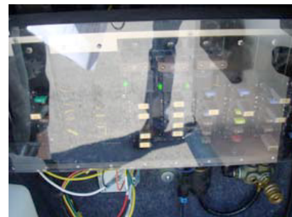
Figure 7-15. Fuse Blocks in exterior compartment on driver's side
