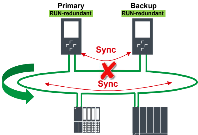
Failure of the direct redundancy connection
