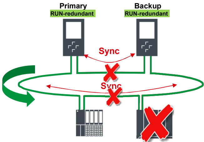
Failure of the two direct redundancy connections and PROFINET cable in the PROFINET ring
