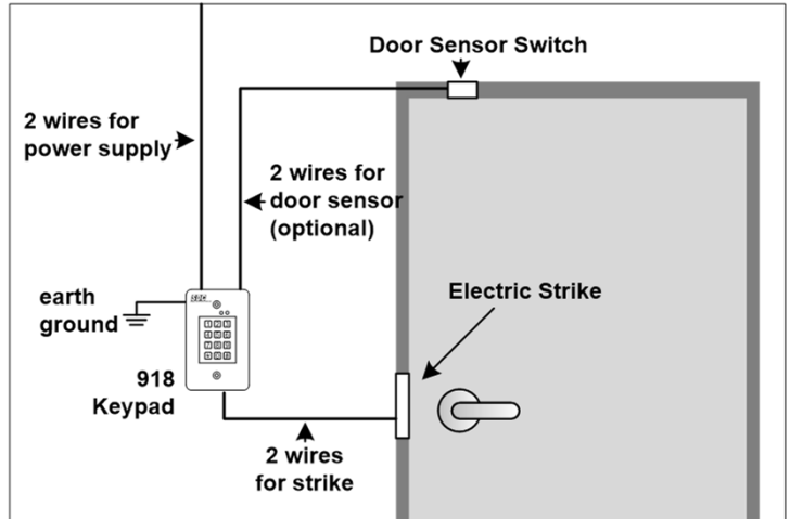
Fig. 3 Typical Door Installation
