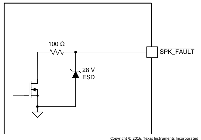
Figure 16. SPK_FAULT Pin
