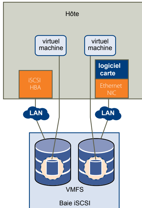
Figure 8-3. Stockage iSCSI
