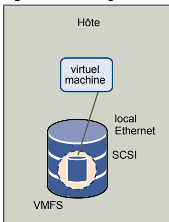
Figure 8-1. Stockage local
