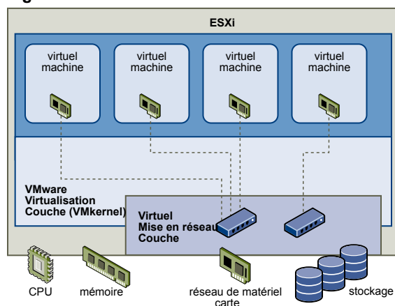
Figure 11-1. Architecture ESXi
