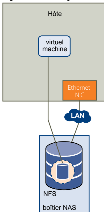
Figure 8-4. Stockage NFS
