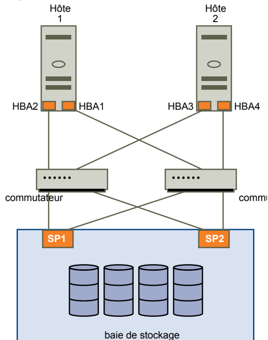
Figure 9-2. Chemins multiples Fibre Channel
