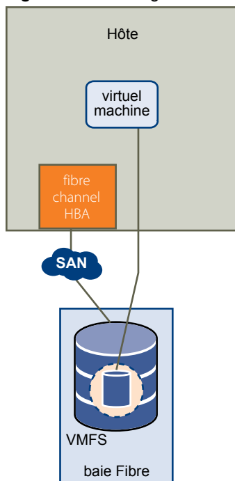
Figure 8-2. Stockage Fibre Channel
