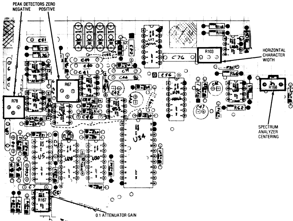
Figure 5-15. Scope/DVM Control Alignment Points
