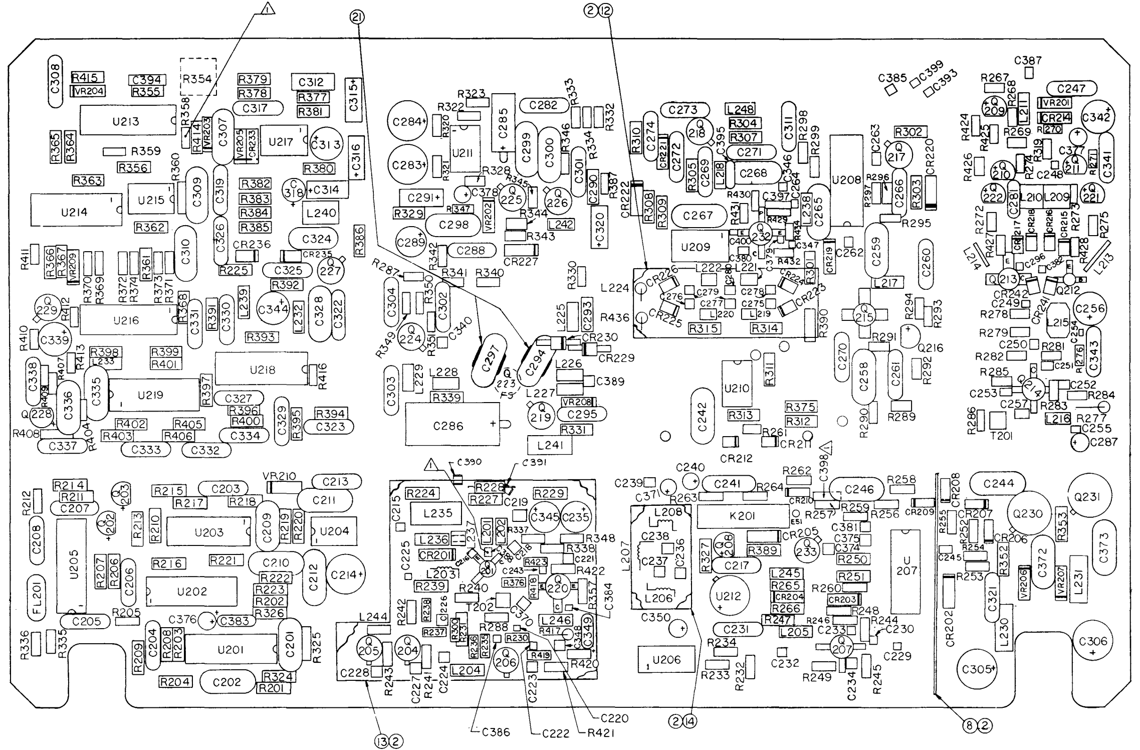
Figure 11-7. RF Synthesizer A5A2 RTC-4010B Parts Location Diagram
