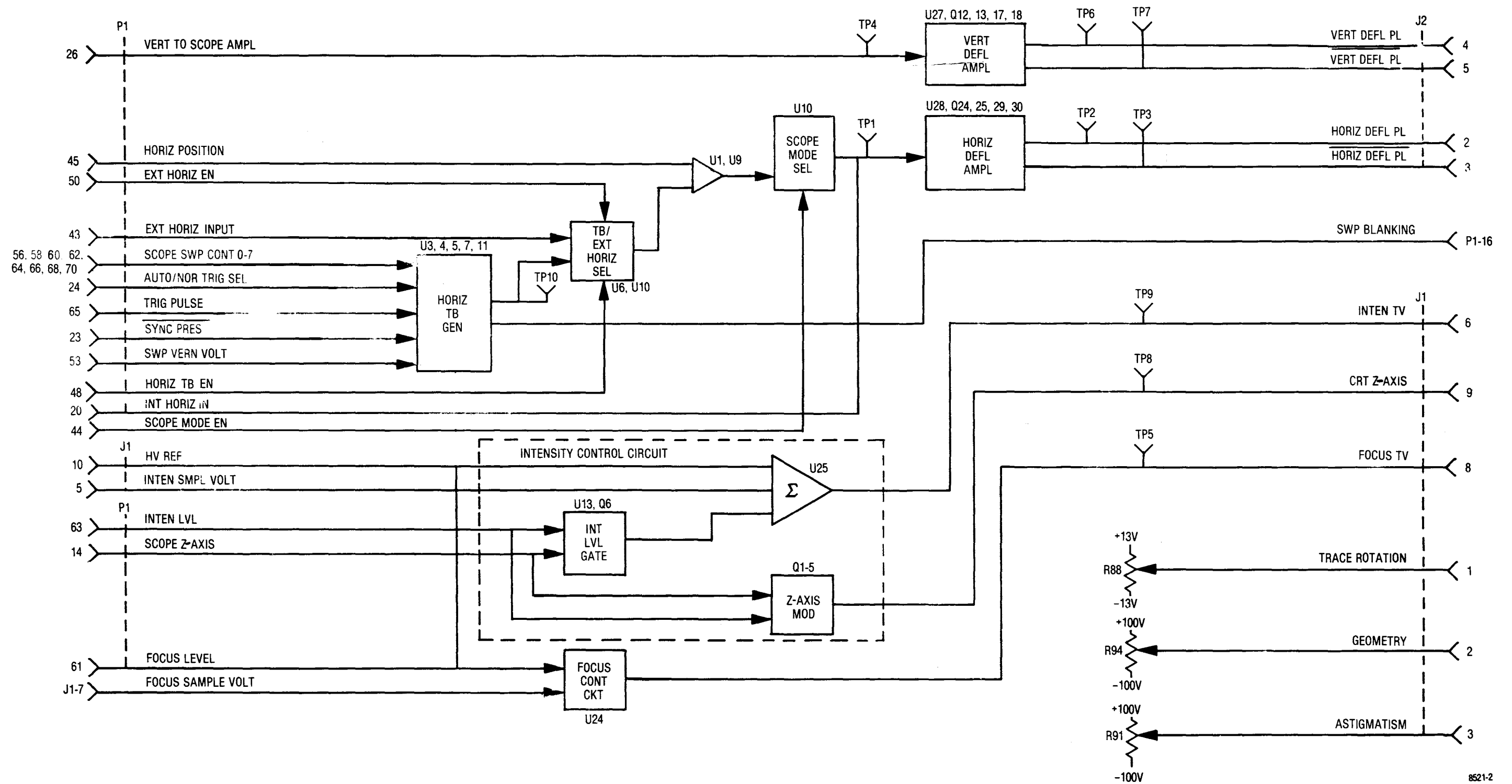
Figure 8-1. Vertical/Horizontal Scope Amplifier A2 Block Diagram
