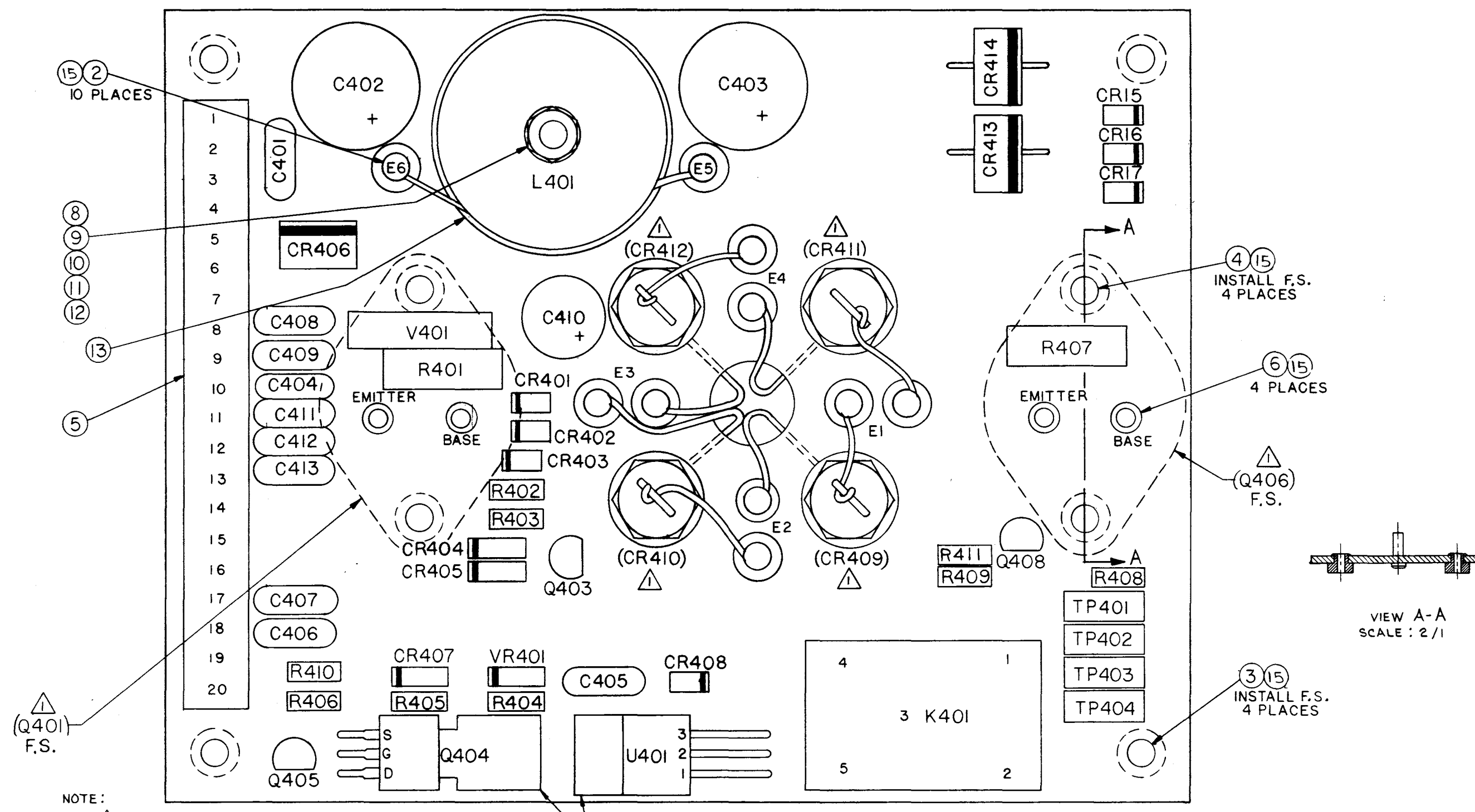
Figure 7-16. Low Voltage Power Supply Relay Module A1A4 (01-80305A68) Parts Location Diagram
