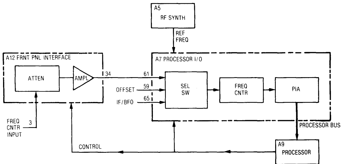
Figure 5-9. Frequency Counter Block Diagram
