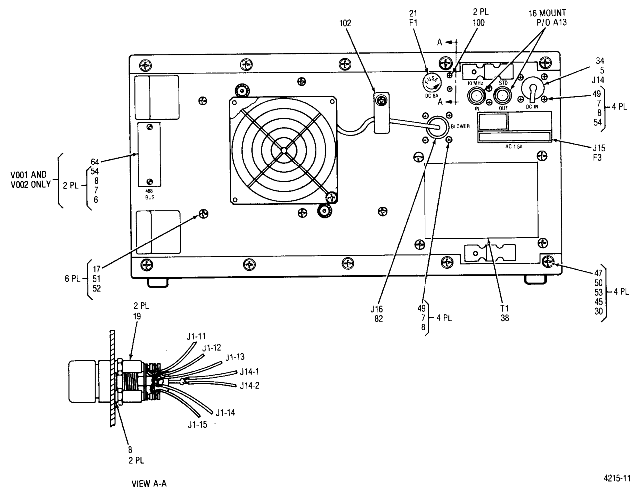
Communications System Analyzer, Rear Panel
