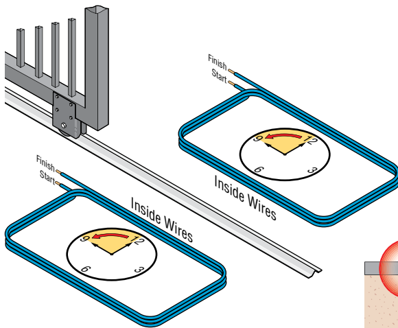
Both loops wound counter-clockwise.
