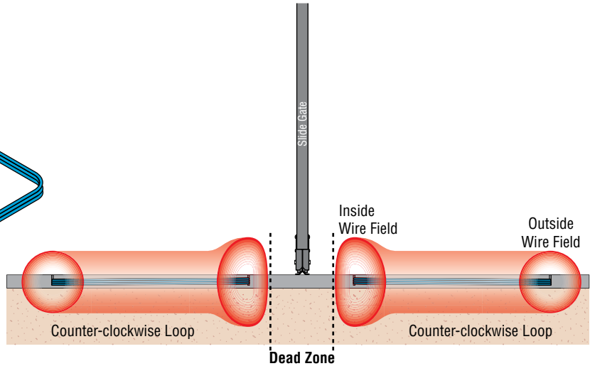
2 loops wound in the same direction repel the inside wire fields.
