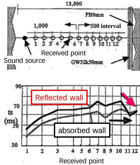
Figure 7: Example of t_s measurement
