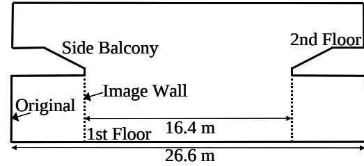
Figure 3: Concept of the Image Wall
