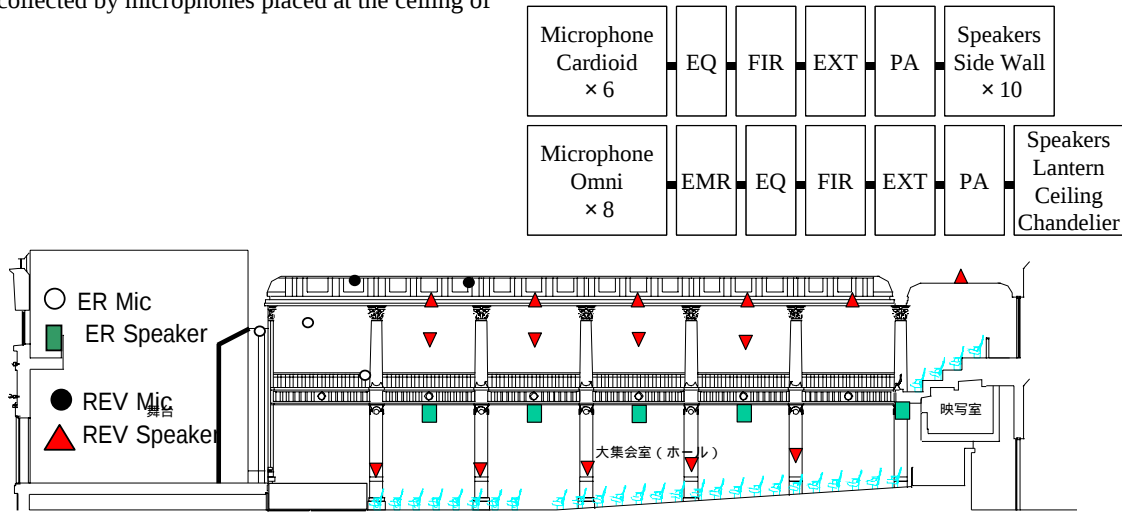
Figure 2: AFC system configuration
