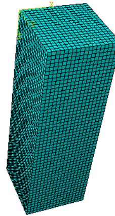
Square cross-section
