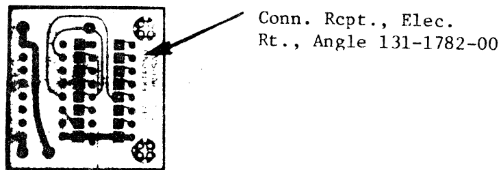
BACK VIEW OF CIRCUIT BOARD
