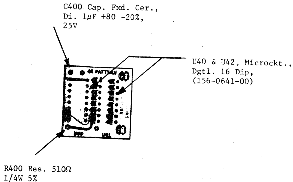
FRONT VIEW OF CIRCUIT BOARD
