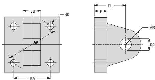
Eye Bracket
