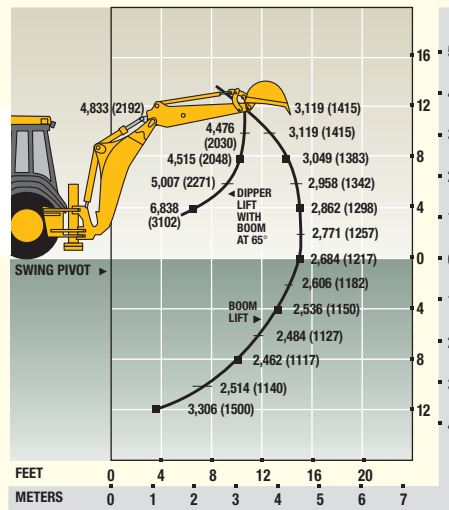
315SG BACKHOE WITH 3-FT. 6-IN. (1.07 M) EXTENDABLE DIPPERSTICK, RETRACTED
