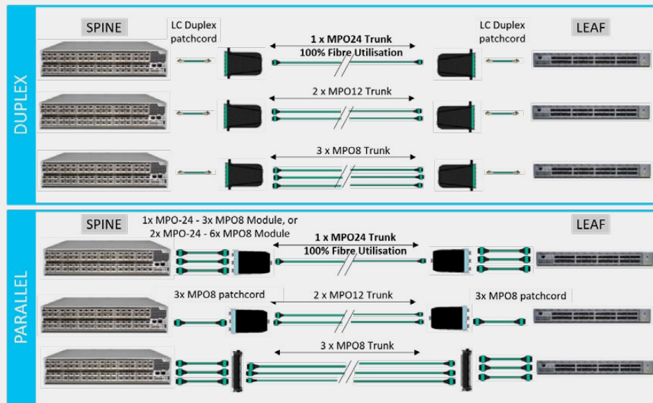
Figure 5: Simple migration using 24-fiber MPO
