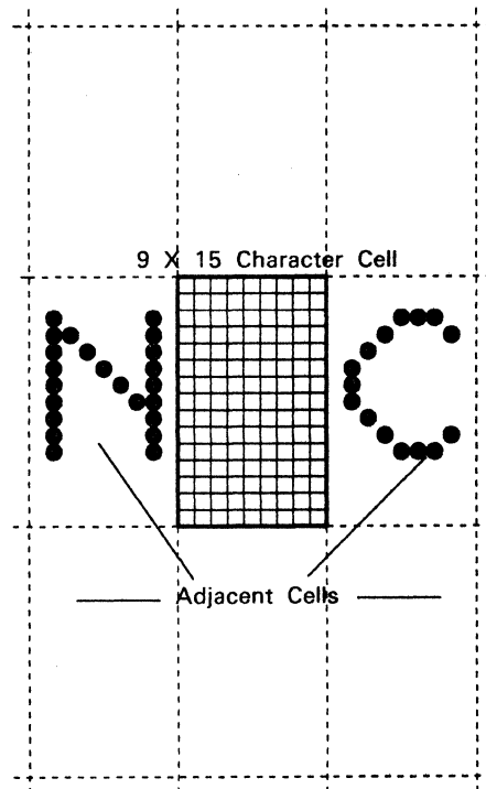
Figure 2-2. Character Cells (9 x 15 Size)
