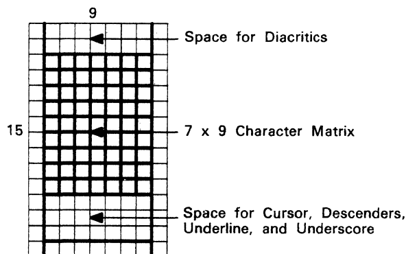
Figure 2-3. 7 x 9 Character Matrix in 9 x 15 Character Cell
