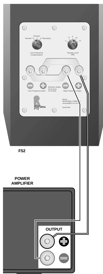
Figure 7: Single-Wired Connections
