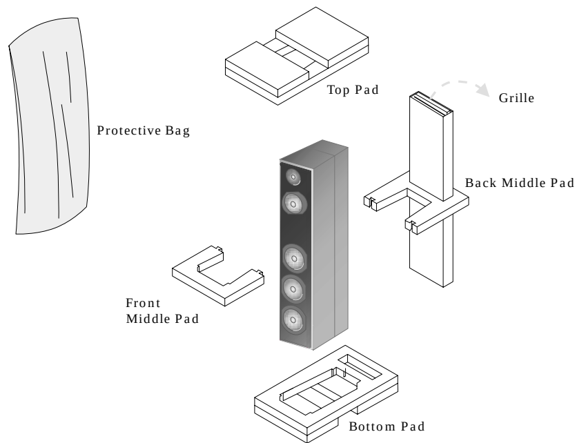
Figure 2: Packing Materials
