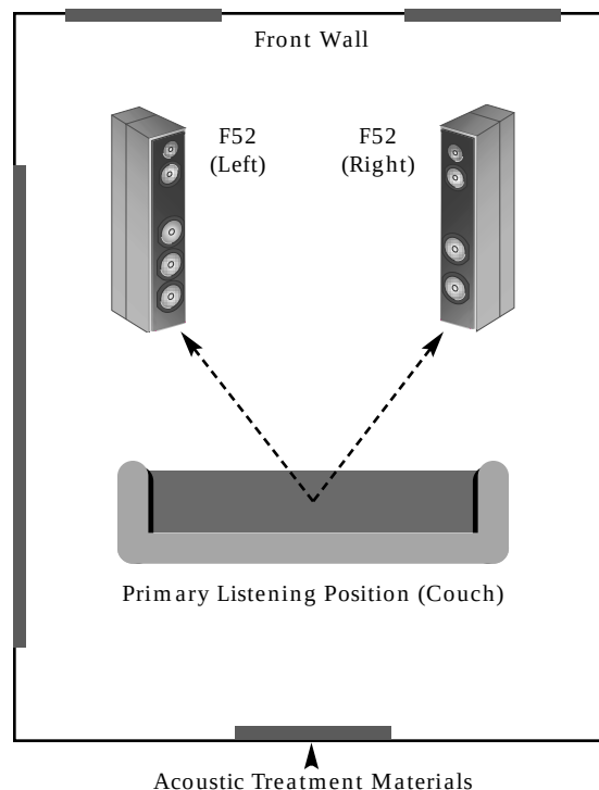
Figure 5: Loudspeaker Placement
