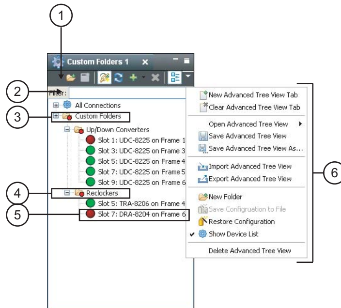
Figure 4.3 Advanced Tree View
