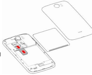
SIM Card
