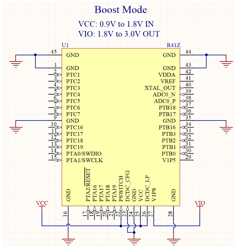
Figure 6 - Schematic: DCDC Boost Mode Example
