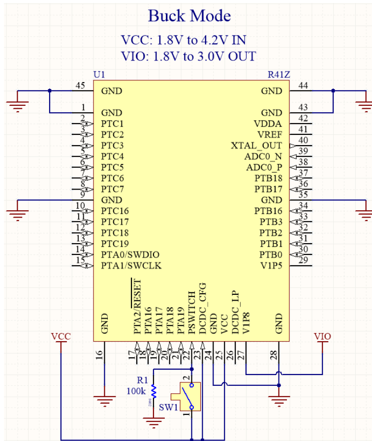
Figure 5 - Schematic: DCDC Buck Mode PSWITCH Example
