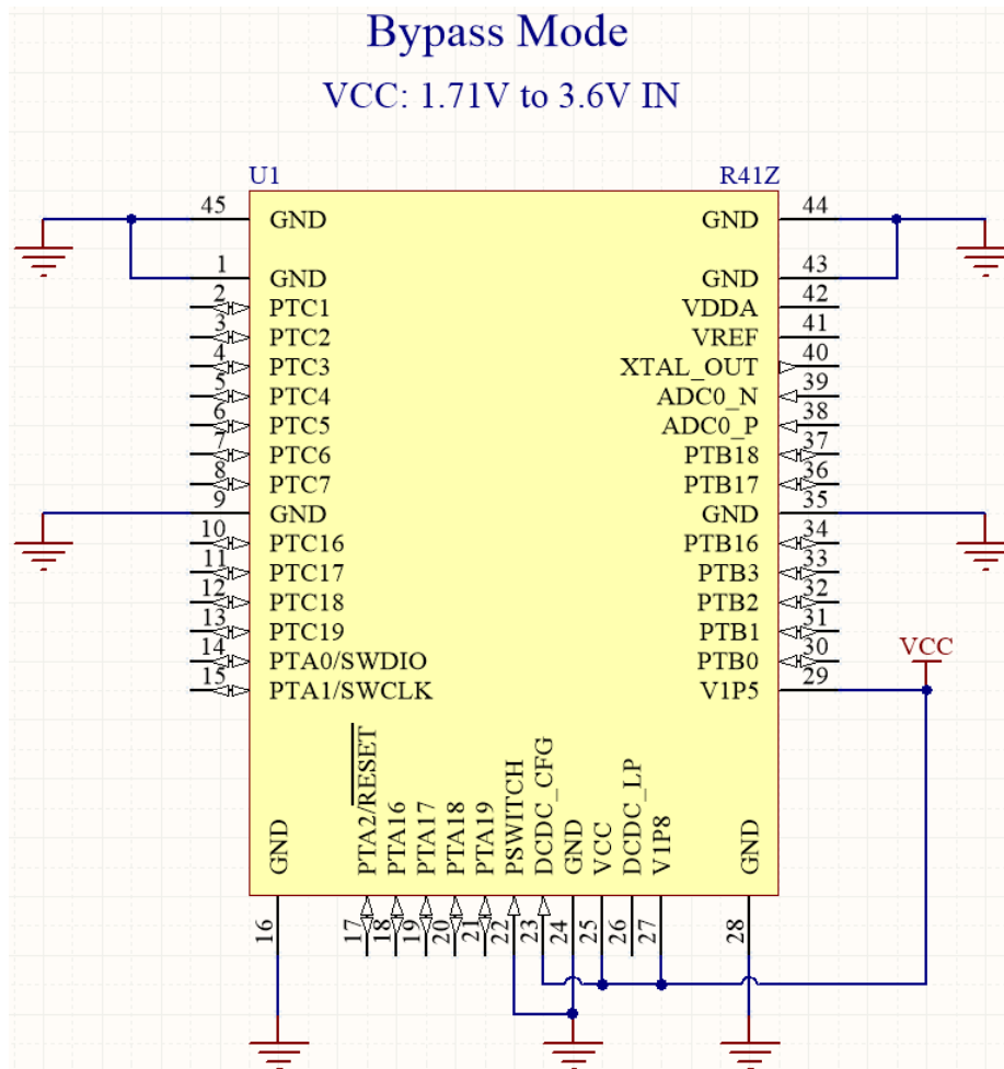
Figure 3 - Schematic: DCDC Bypass Mode Example
