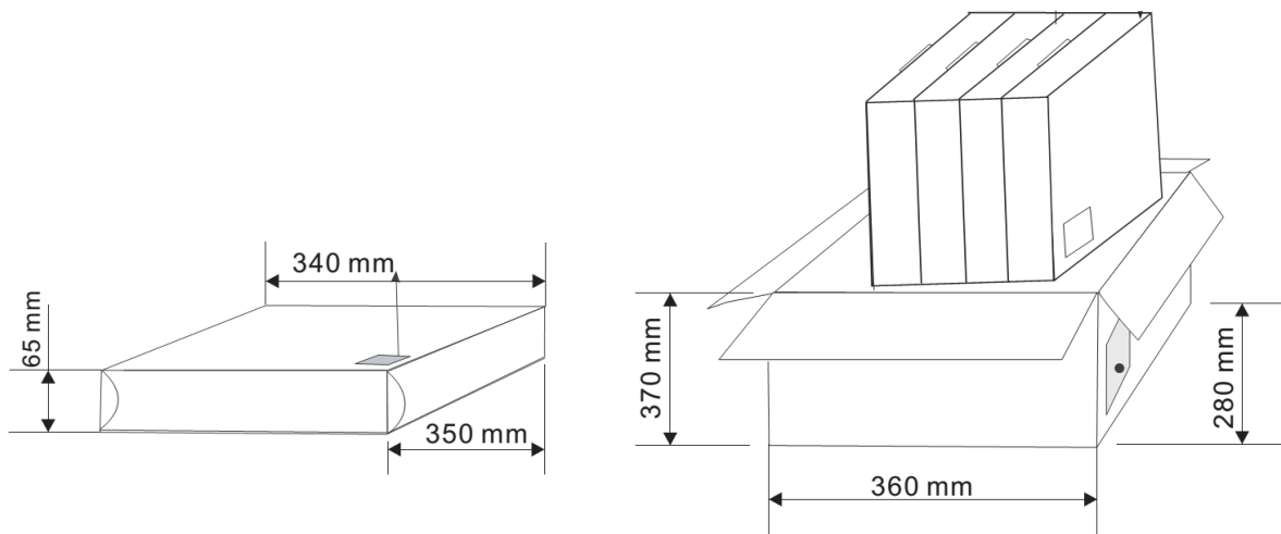
Figure 16 - Reel Cartons
