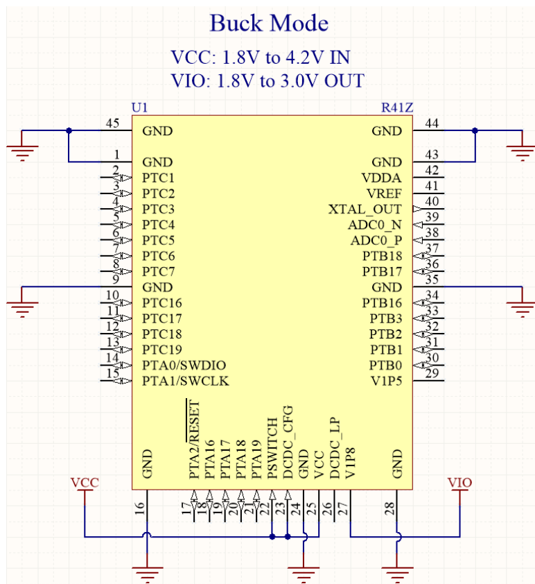
Figure 4 - Schematic: DCDC Buck Mode Example
