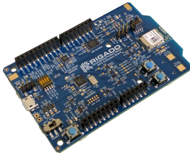
Figure 14 - R41Z Evaluation Board
