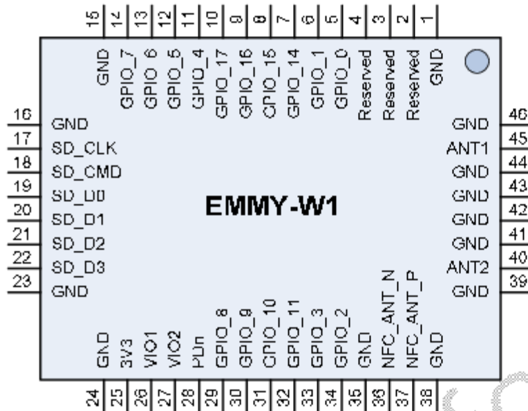
Figure 11: Pin assignment
