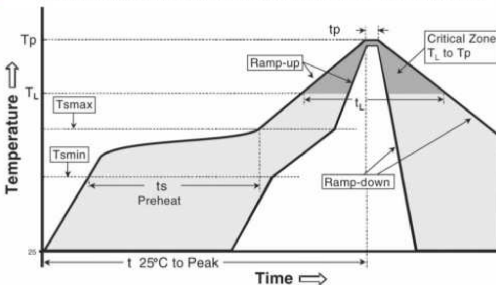
Figure 15: Reflow profile
