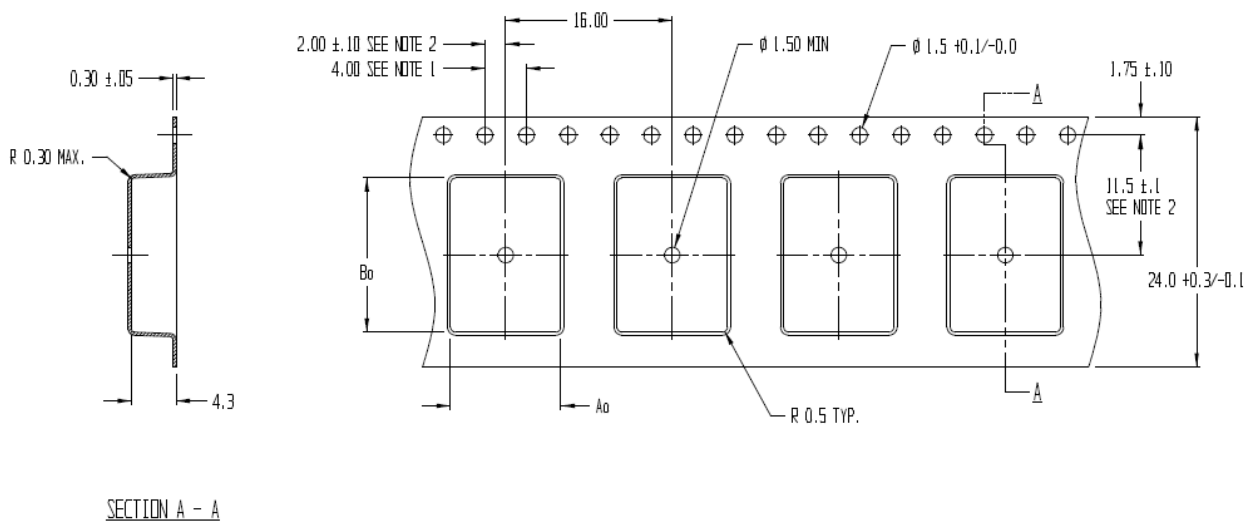
Figure 10: NINA-W131 tape dimension
