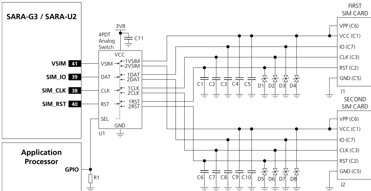
Figure 57: Application circuit for the connection to two removable SIM cards, with SIM detection implemented
