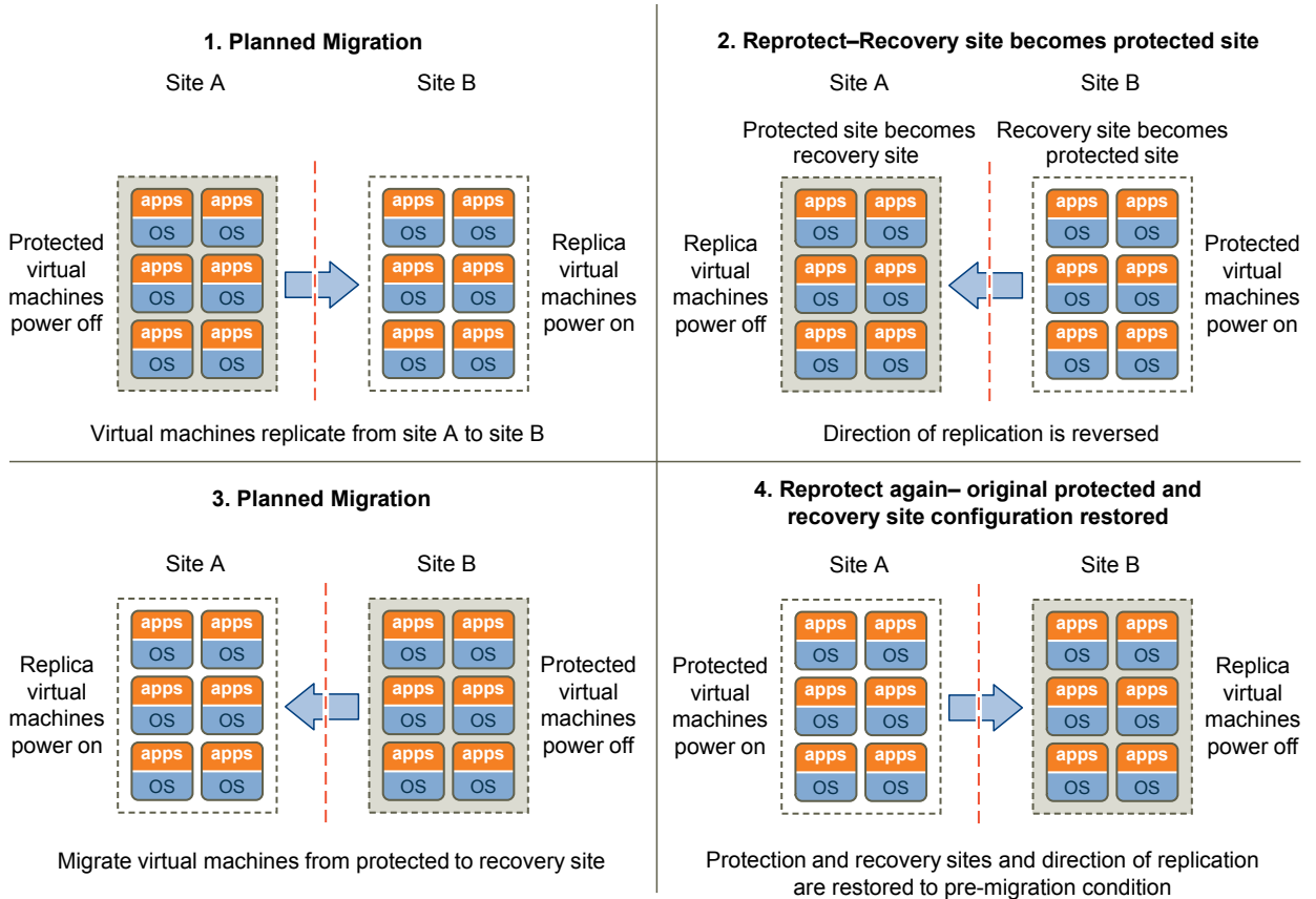
Figure 10-1. Site Recovery Manager Failback Process
