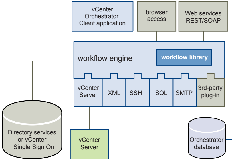
Figure 1-1. VMware vCenter Orchestrator Architecture
