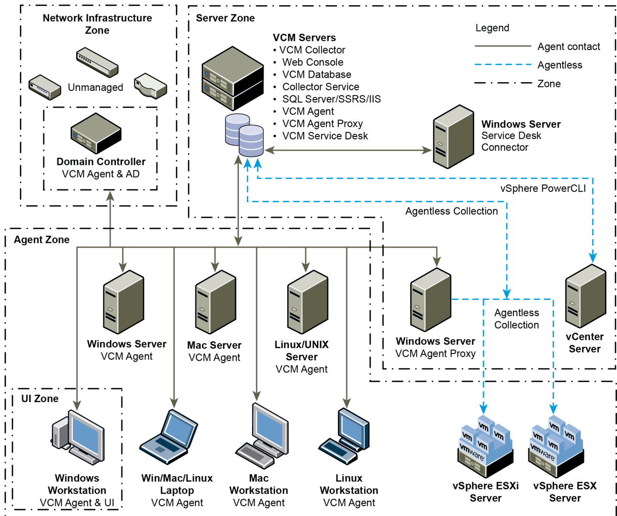
Figure 1–1. VCM Components and Zones
