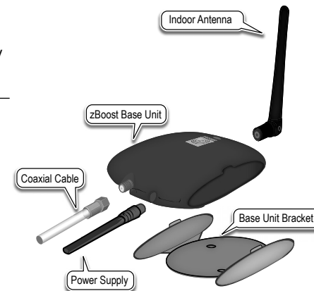
zBoost Base Unit Assembly
