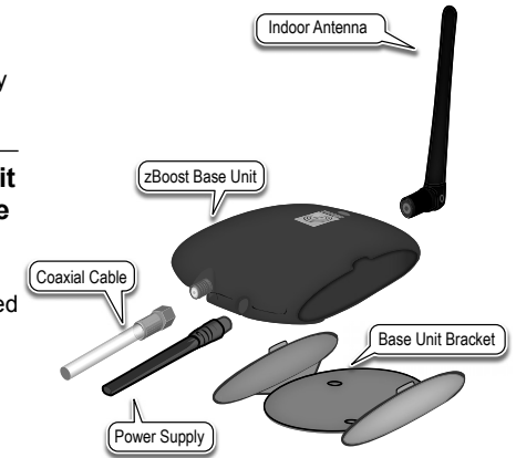
zBoost Base Unit Assembly
